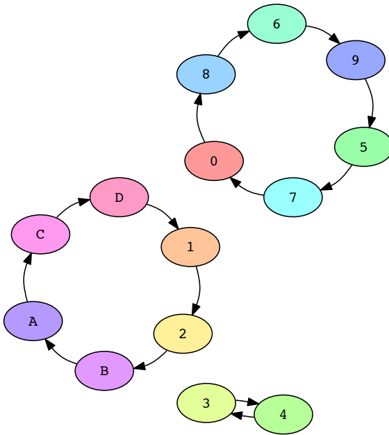
Figure 6.4: An encryption permutation produced by the block cipher under some other key.
