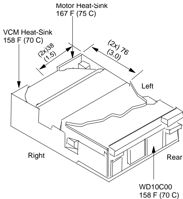
Figure 3 Temperature Measurement Points
